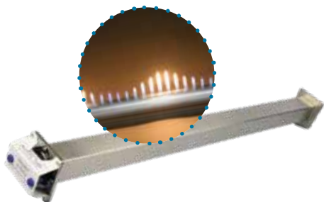
RUBENS TUBE [105089]
