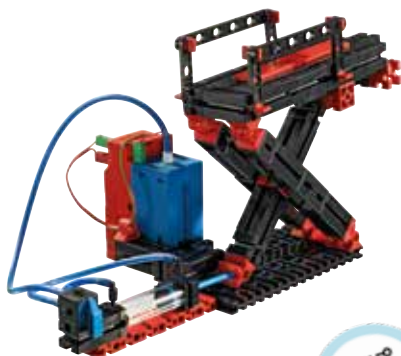
FISHERTECHNIK PNEUMATICS (101468)
